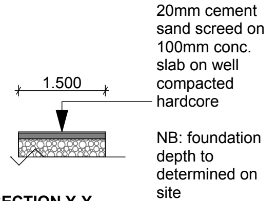
SECTION Y-Y
